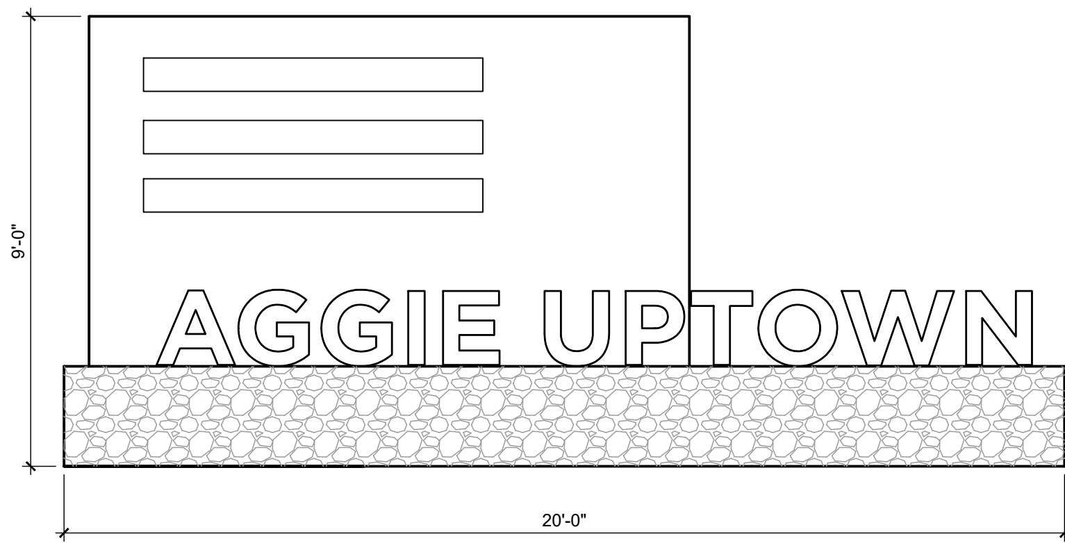
C2 SECONDARY ENTRANCE SIGN B 3/8" = 1'-0"
