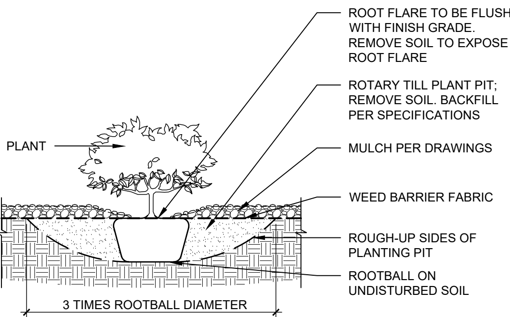
XX SHRUB IN BED 3/4" = 1'-0"
