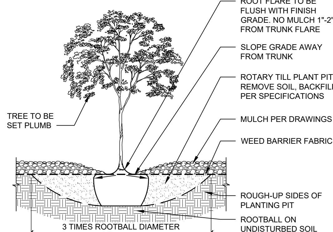
XX TREE IN PLANTING BED 3/4" = 1'-0"
