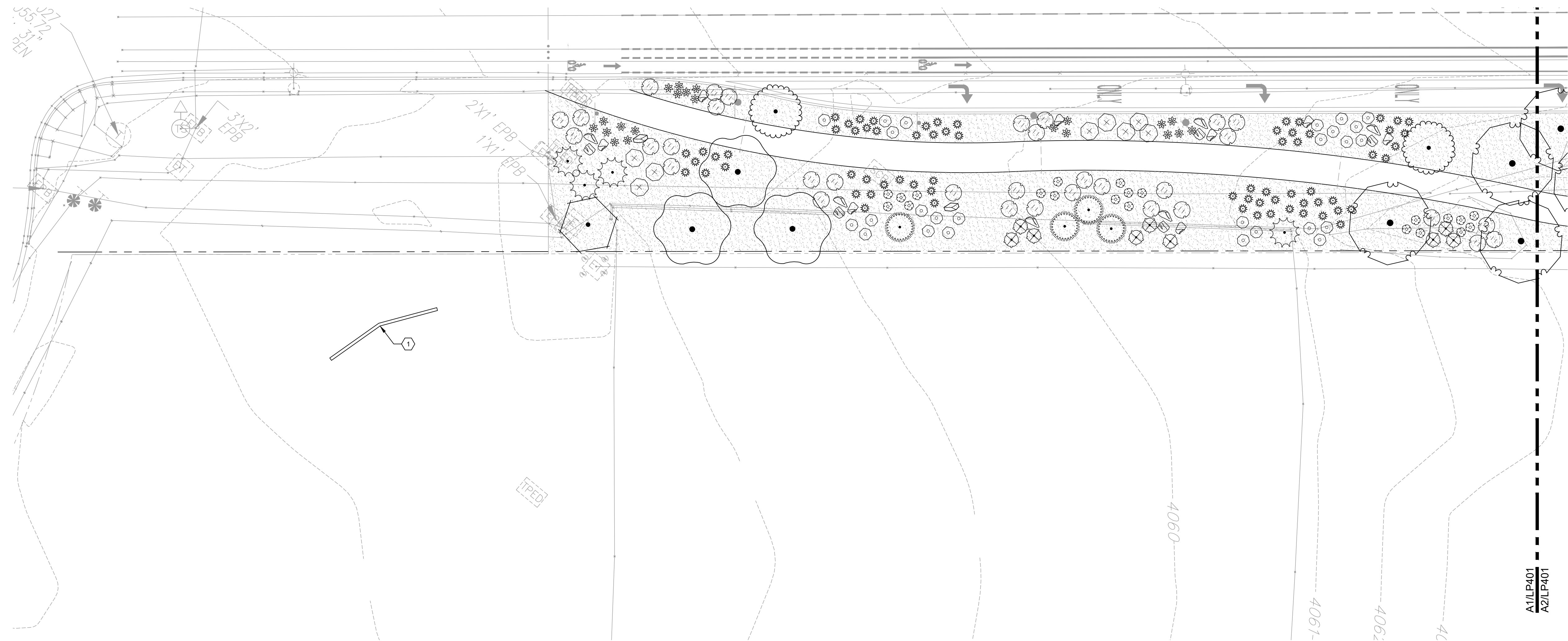
A1 LANDSCAPE PLAN 1" = 20'-0" 0 10' 20' 40'
